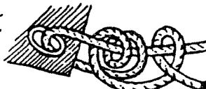
TAUT-LINE HITCH
